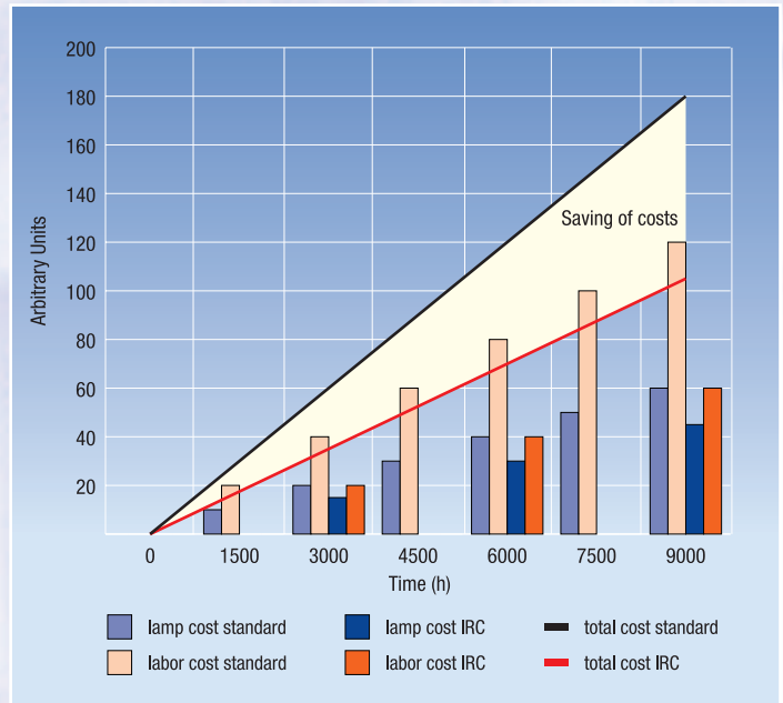
Figure 1: Accumulated saving of costs (through extended replacement intervals) when using IRC-Airfield lamps instead of standard lamps
