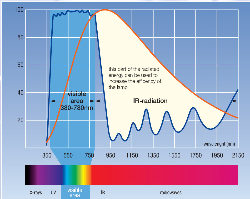
Figure 2: IRC-Airfield lamps, sphere of activity
